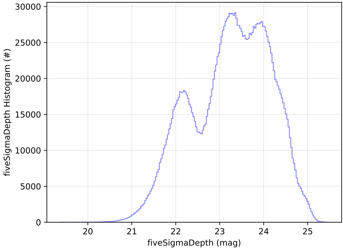
ddf_acor_sf10_lsf30_lsr50_v3.4_10yrs WFD all bands: fiveSigmaDepth Histogram
