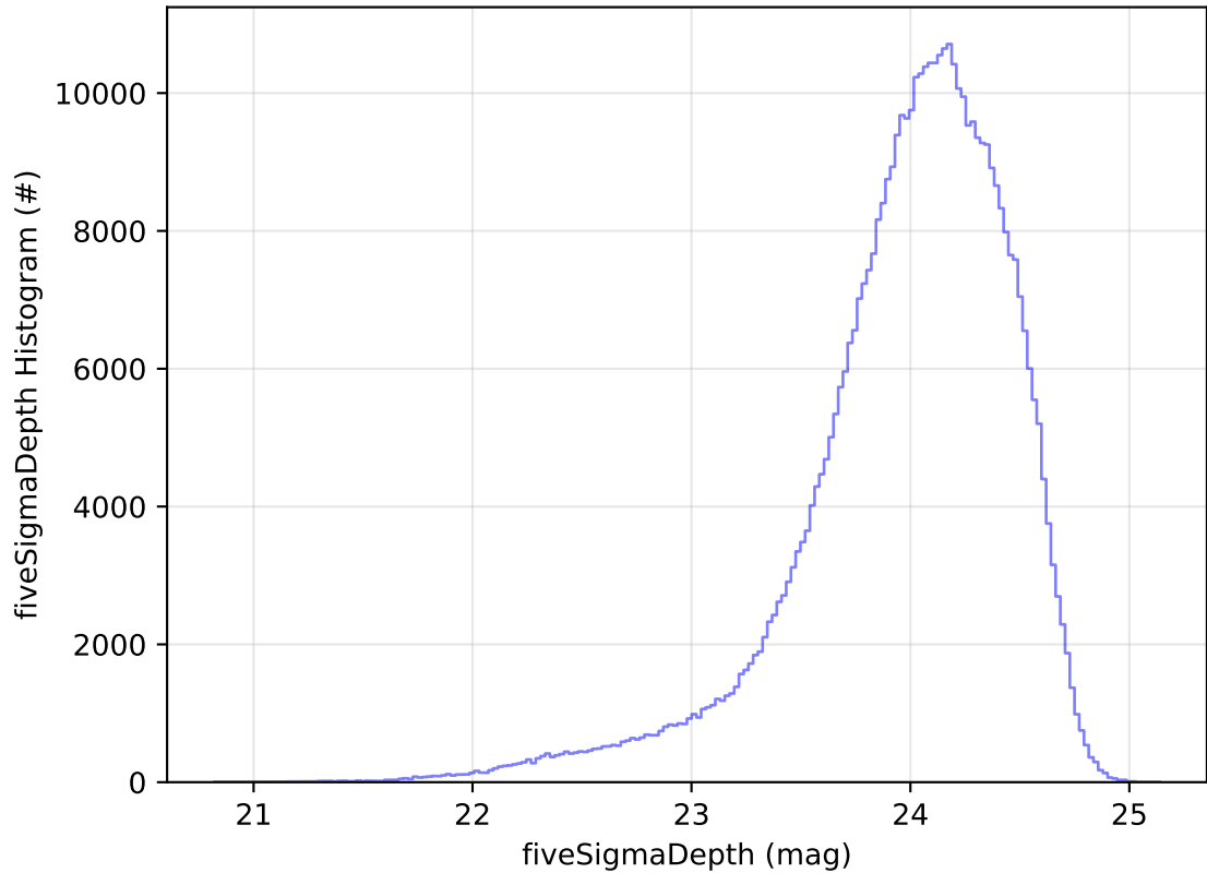
ddf_acor_sf10_ls30_lsr50_v3.4_10yrs All sky r band: fiveSigmaDepth Histogram
