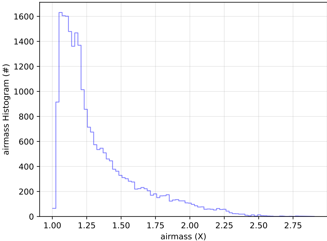
ddf_acor_sf10_lsf30_lsr50_v3.4_10yrs Yr 1 g band: airmass Histogram
