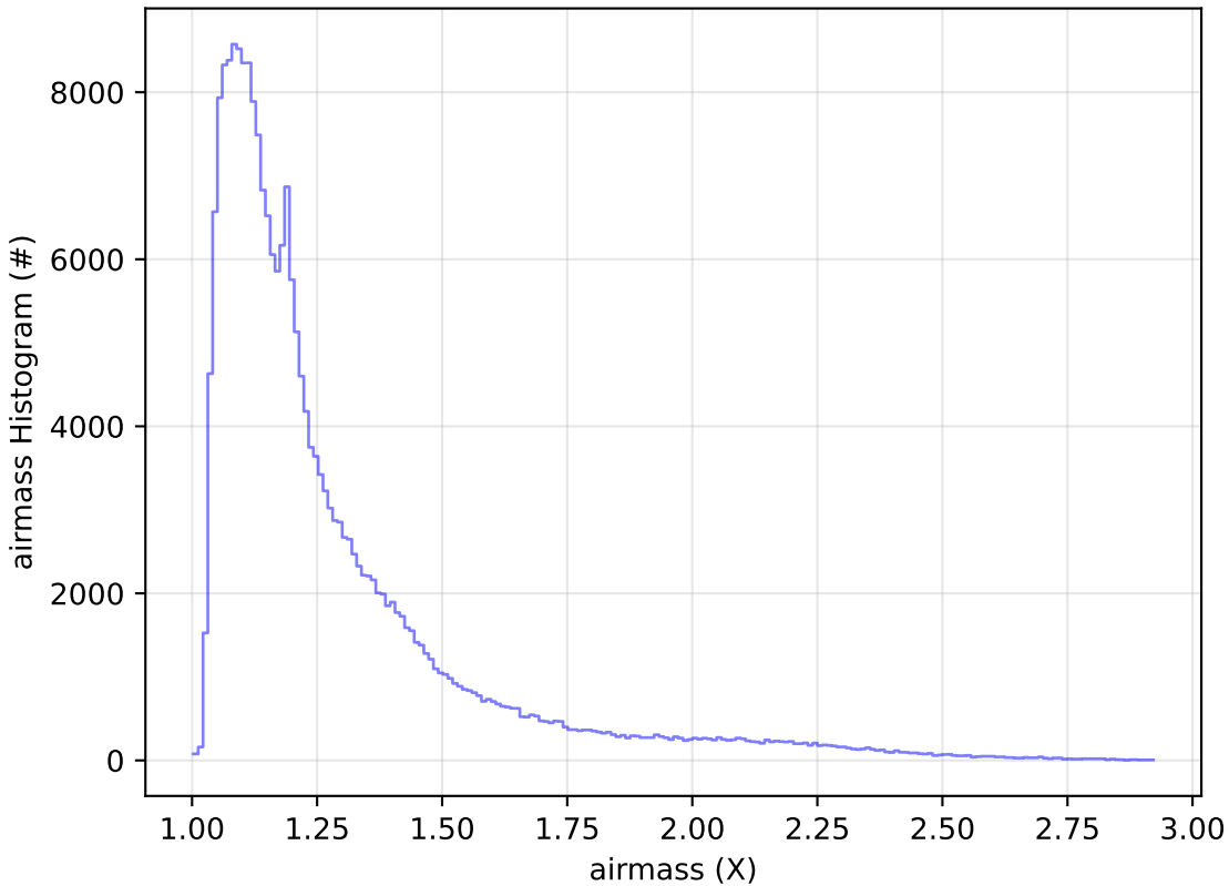
ddf_acor_sf10_lsf30_lsr50_v3.4_10yrs Yr 1 all bands: airmass Histogram
