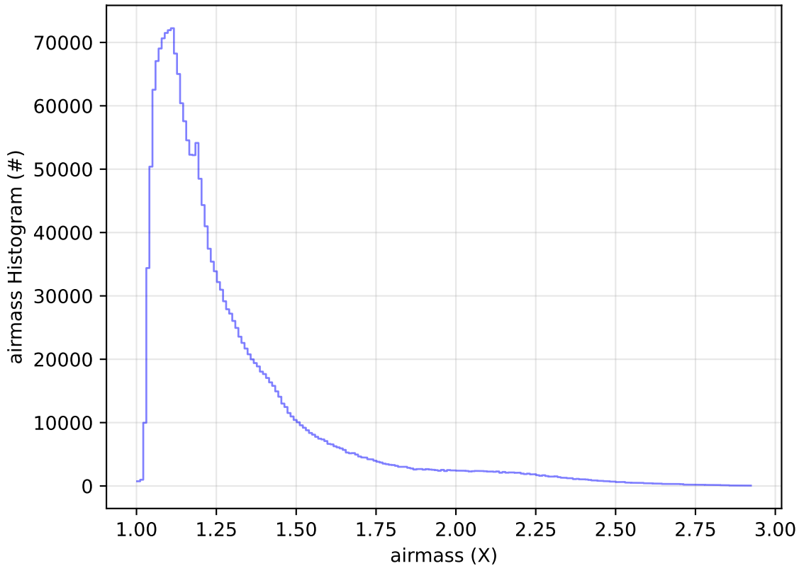
ddf_acor_sf10_lsf30_lsr50_v3.4_10yrs WFD all bands: airmass Histogram
