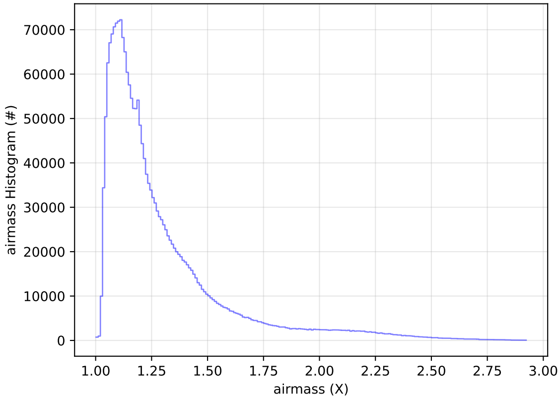
ddf_acor_sf10_lsf30_lsr50_v3.4_10yrs All sky all bands: airmass Histogram
