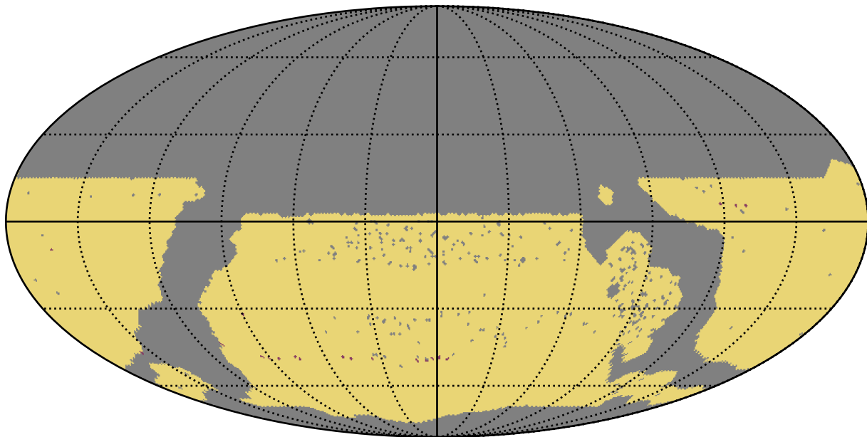
ddf_acor_sf10_lsf30_lsr50_v3.4_10yrs WFD: RapidRevisits
