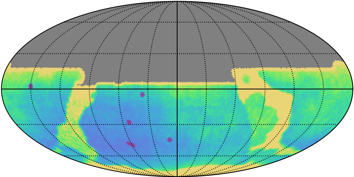
ddf_acor_sf10_lsf30_lsr50_v3.4_10yrs All sky y band only: Parallax Uncert @ 21.3
