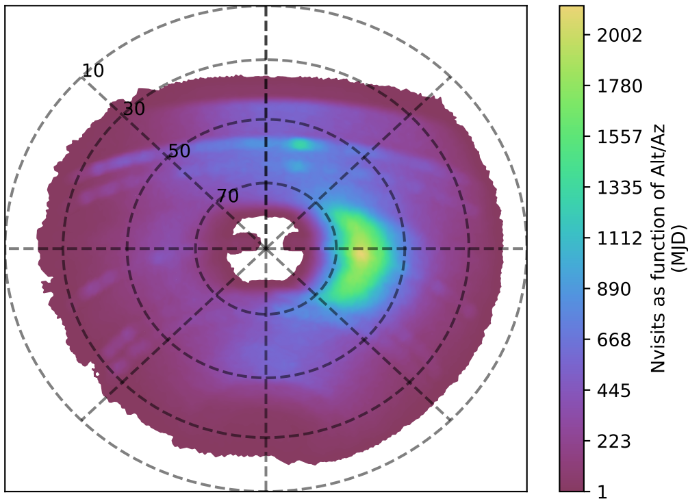
ddf_acor_sf10_lsf30_lsr50_v3.4_10yrs y band: Nvisits as function of Alt/Az
