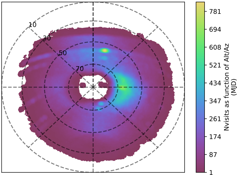
ddf_acor_sf10_lsf30_lsr50_v3.4_10yrs u band: Nvisits as function of Alt/Az
