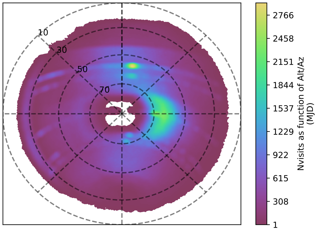
ddf_acor_sf10_lsf30_lsr50_v3.4_10yrs r band: Nvisits as function of Alt/Az
