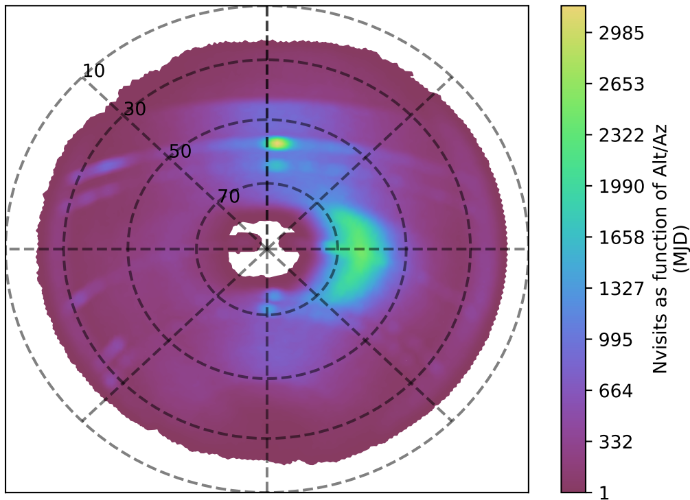
ddf_acor_sf10_lsf30_lsr50_v3.4_10yrs i band: Nvisits as function of Alt/Az
