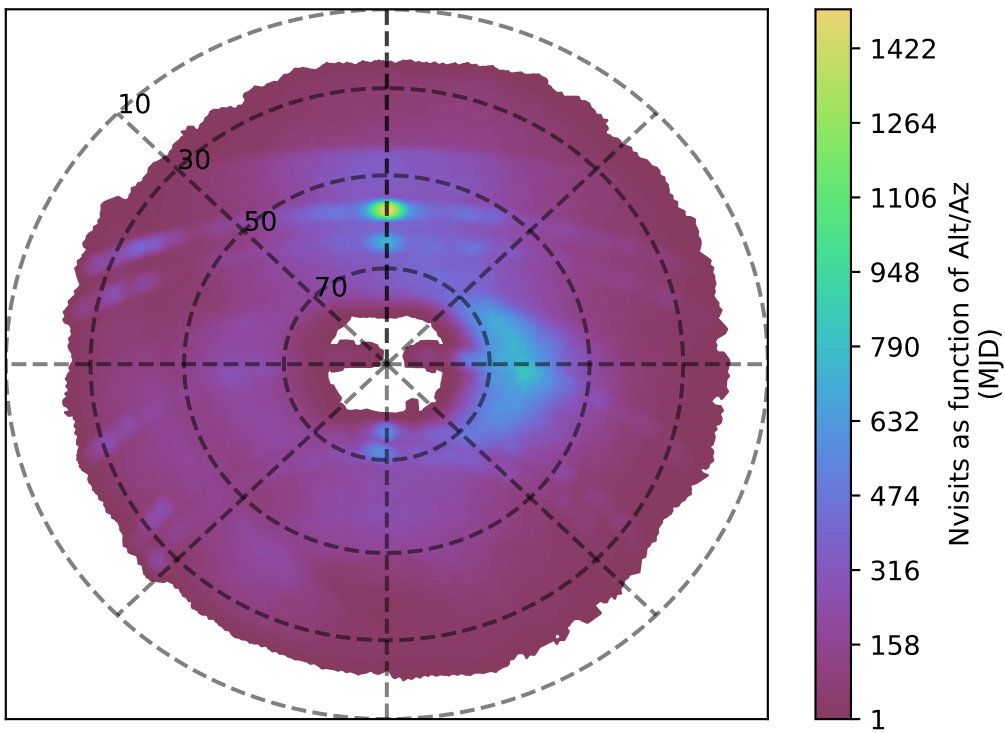
ddf_acor_sf10_lsf30_lsr50_v3.4_10yrs g band: Nvisits as function of Alt/Az
