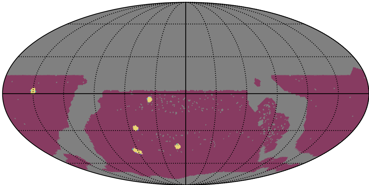
ddf_acor_sf10_lsf30_lsr50_v3.4_10yrs WFD: NumberOfQuickRevisits
