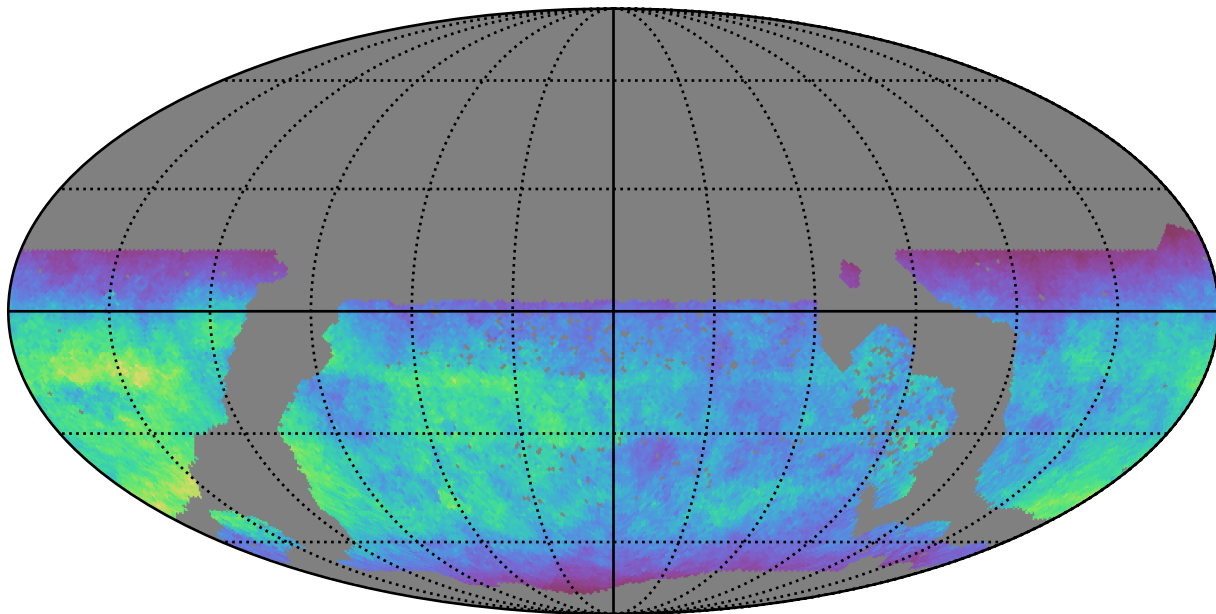
ddf_acor_sf10_lsf30_lsr50_v3.4_10yrs WFD u band: Normalized Teff
