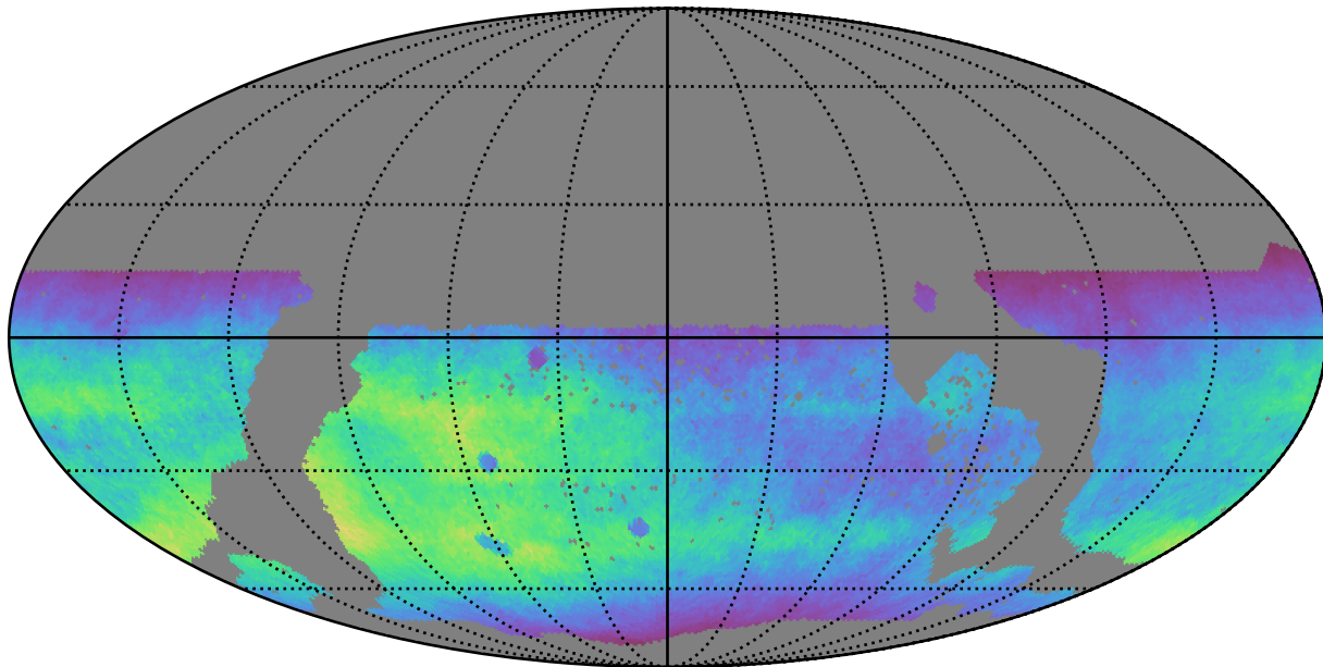
ddf_acor_sf10_lsf30_lsr50_v3.4_10yrs WFD r band: Normalized Teff
