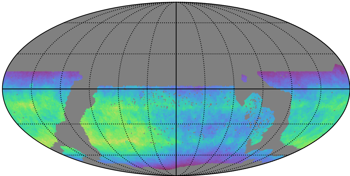
ddf_acor_sf10_lsf30_lsr50_v3.4_10yrs WFD i band: Normalized Teff
