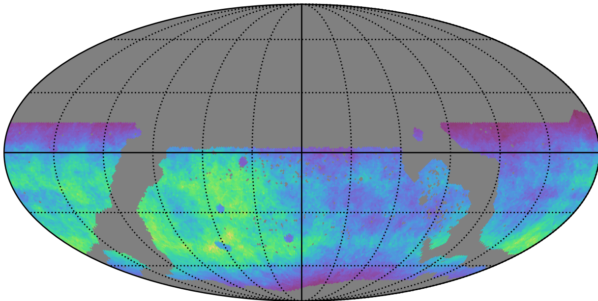
ddf_acor_sf10_lsf30_lsr50_v3.4_10yrs WFD g band: Normalized Teff
