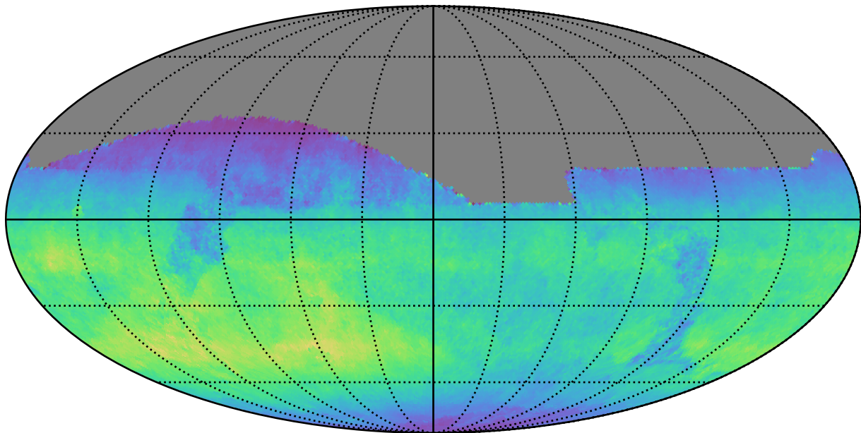
ddf_acor_sf10_lsf30_lsr50_v3.4_10yrs All sky z band: Normalized Teff
