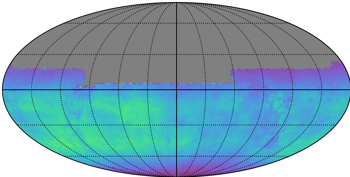
ddf_acor_sf10_lsf30_lsr50_v3.4_10yrs All sky y band: Normalized Teff
