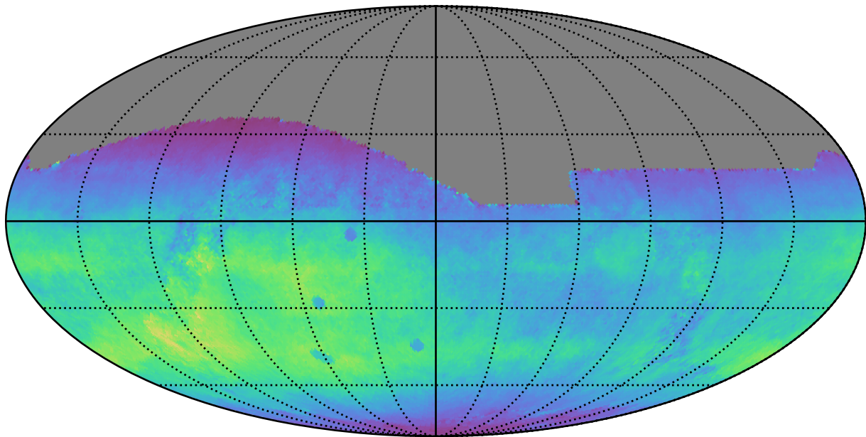
ddf_acor_sf10_lsf30_lsr50_v3.4_10yrs All sky r band: Normalized Teff
