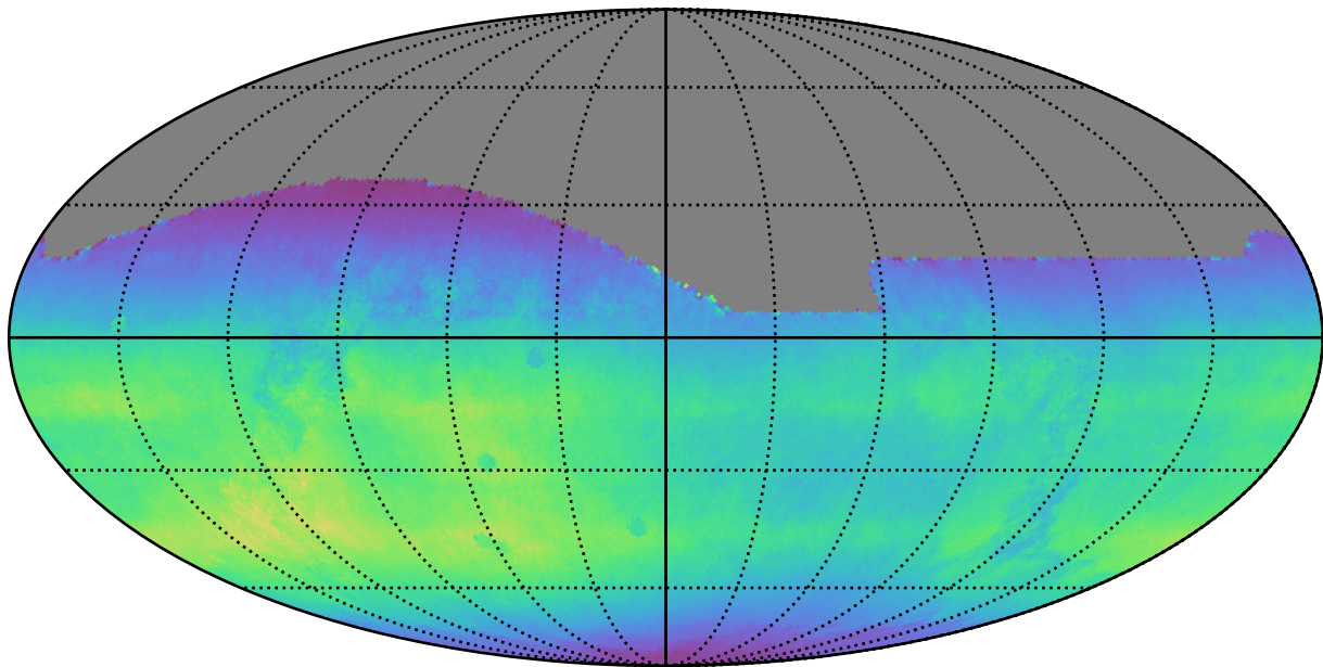
ddf_acor_sf10_lsf30_lsr50_v3.4_10yrs All sky all bands: Normalized Teff
