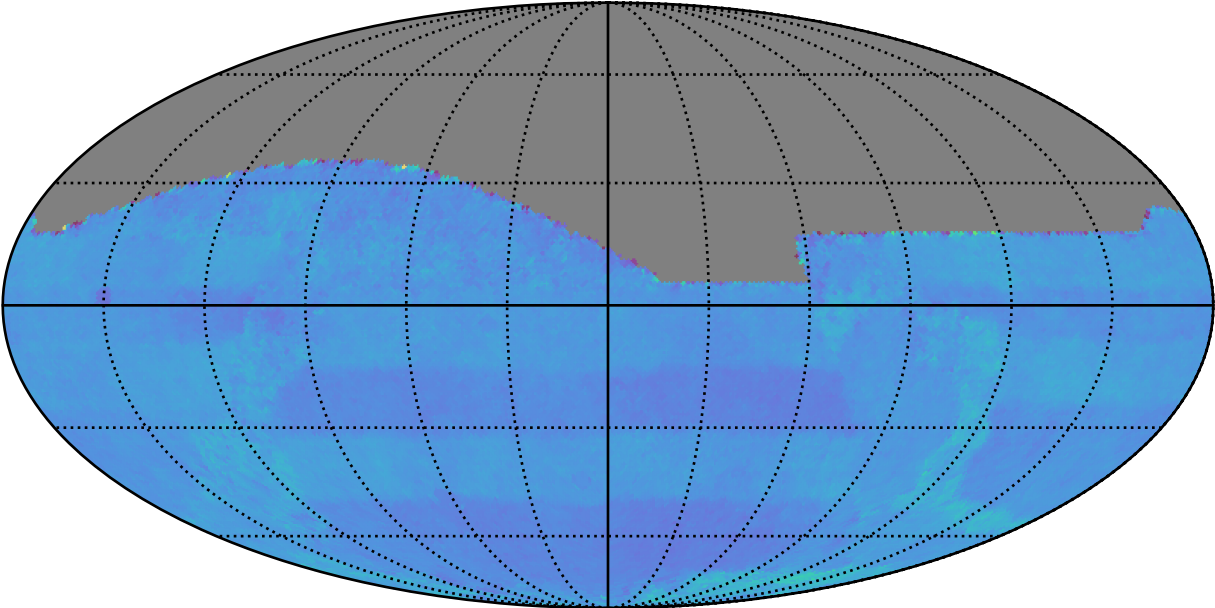
ddf_acor_sf10_lsf30_lsr50_v3.4_10yrs All sky: Normalized Proper Motion Uncert @ 24.0
