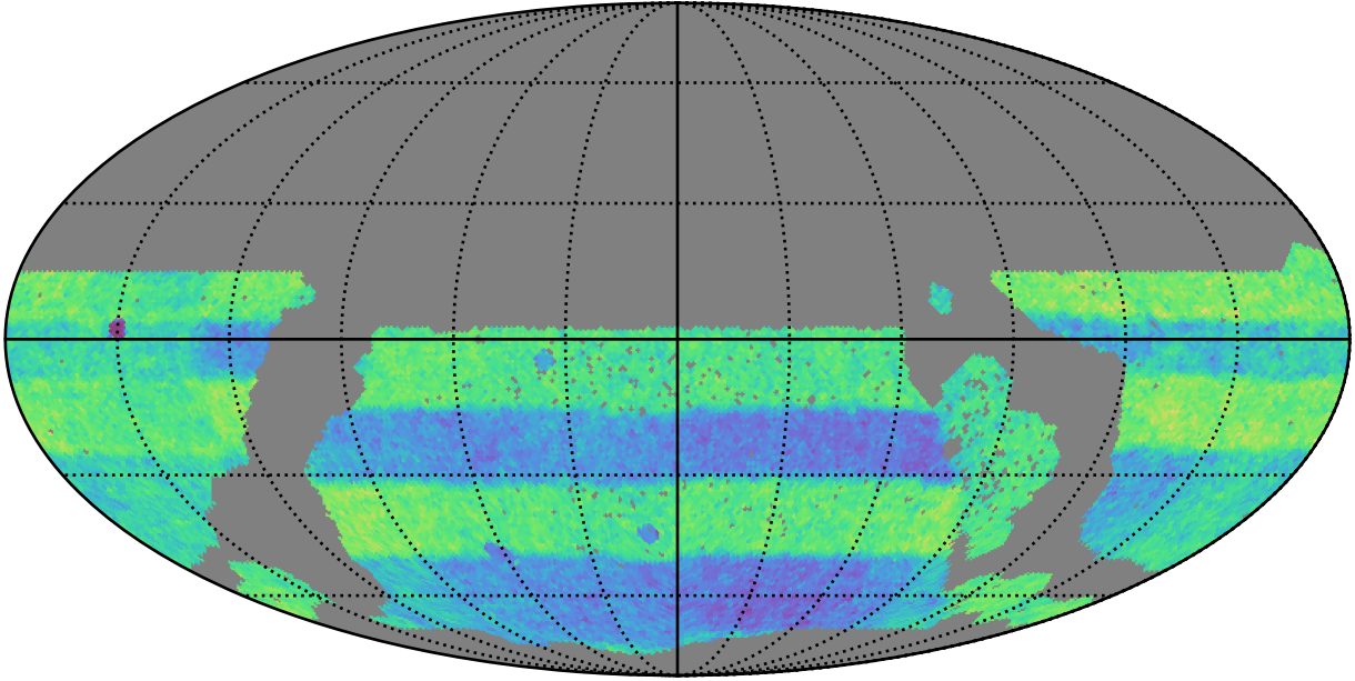
ddf_acor_sf10_lsf30_lsr50_v3.4_10yrs WFD: Normalized Proper Motion Uncert @ 20.5
