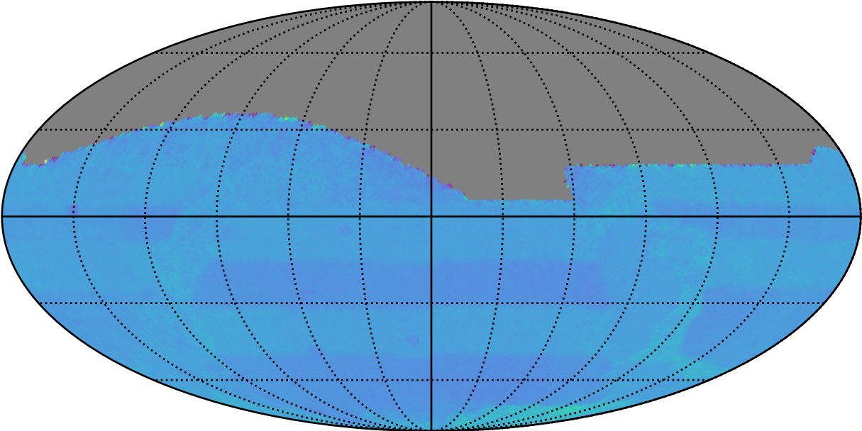
ddf_acor_sf10_lsf30_lsr50_v3.4_10yrs All sky: Normalized Proper Motion Uncert @ 20.5
