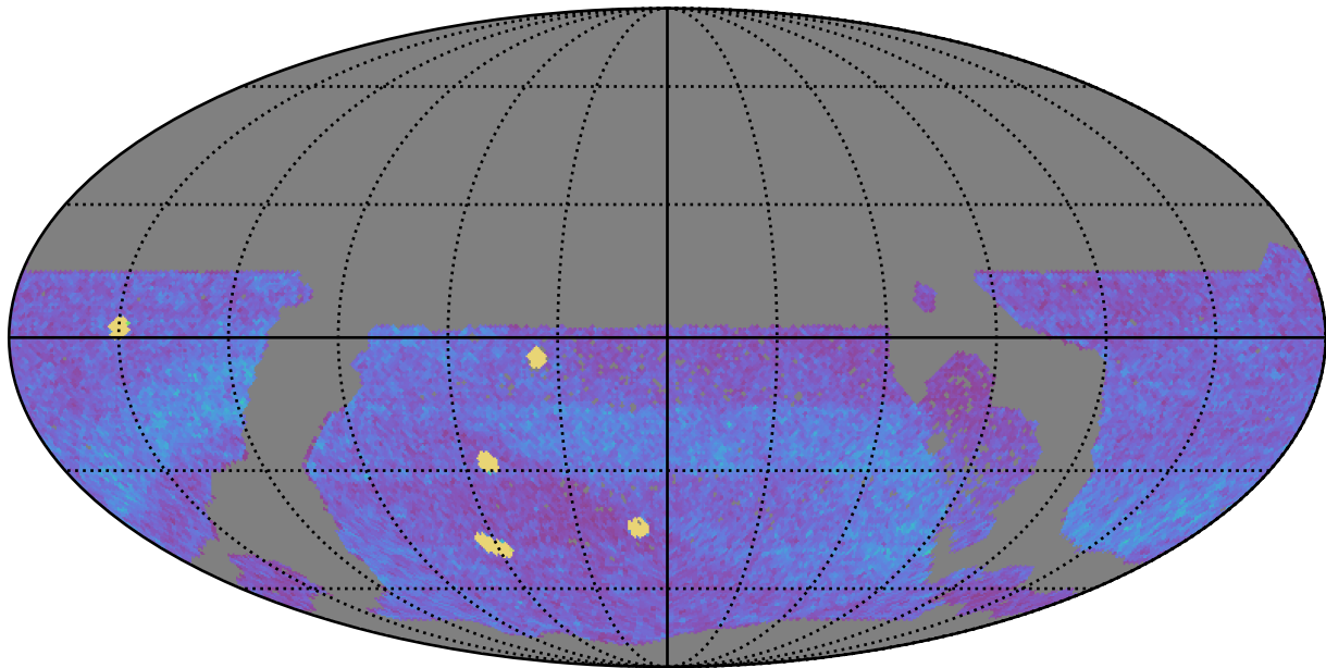
ddf_acor_sf10_lsf30_lsr50_v3.4_10yrs WFD all bands: NVisits
