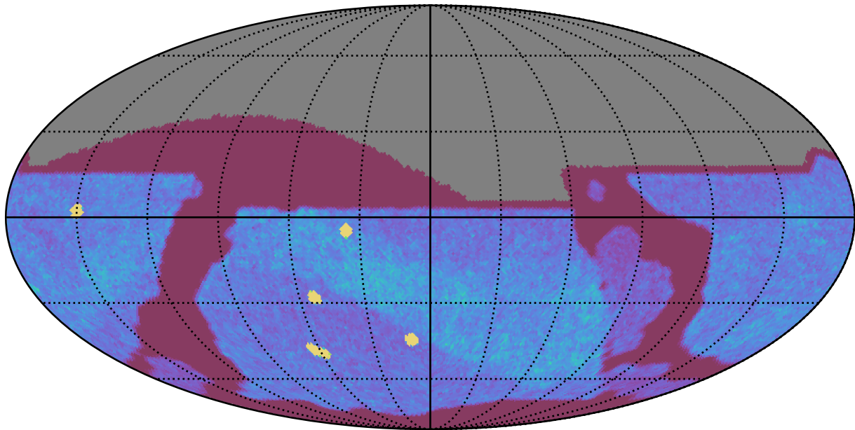
ddf_acor_sf10_lsf30_lsr50_v3.4_10yrs All sky z band: NVisits
