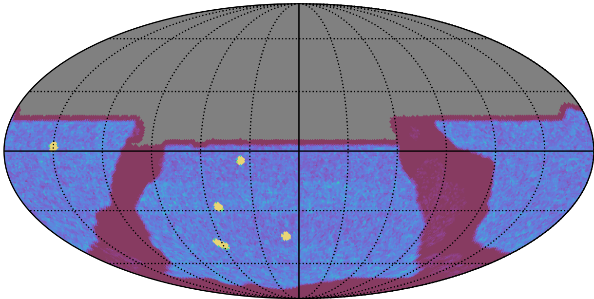
ddf_acor_sf10_lsf30_lsr50_v3.4_10yrs All sky y band: NVisits
