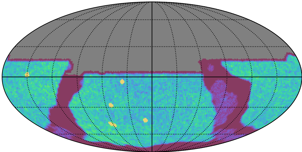
ddf_acor_sf10_lsf30_lsr50_v3.4_10yrs All sky u band: NVisits
