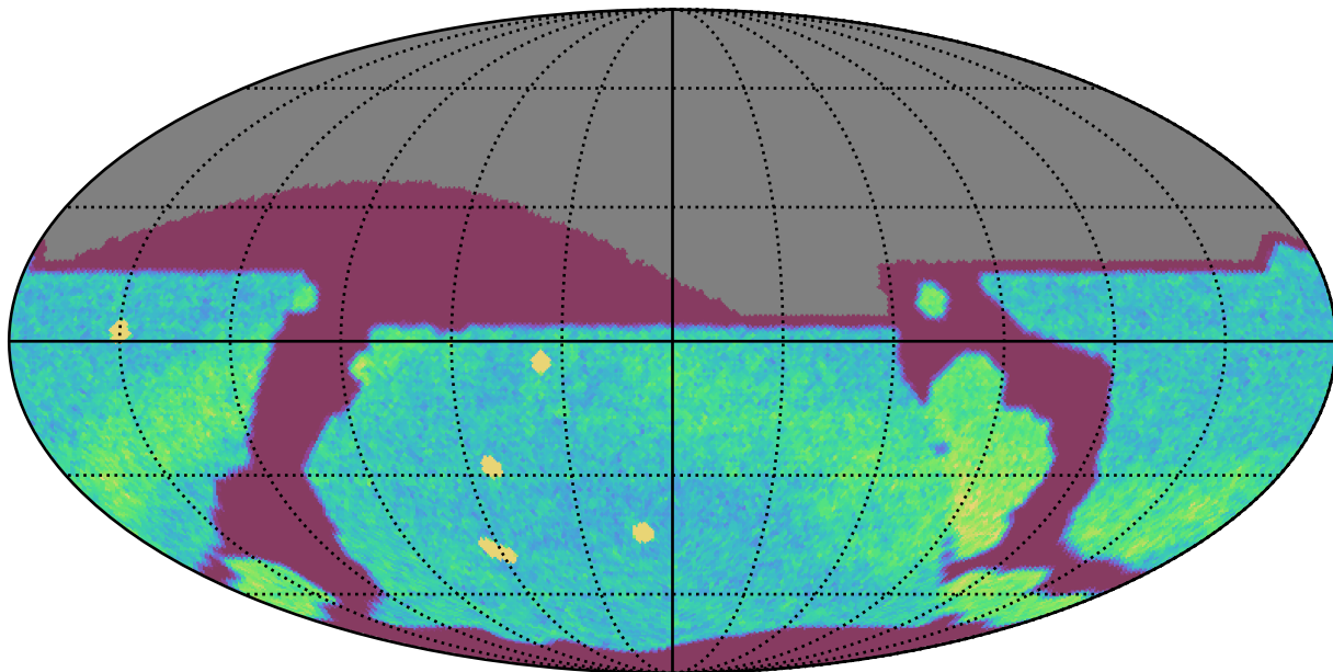
ddf_acor_sf10_lsf30_lsr50_v3.4_10yrs All sky r band: NVisits
