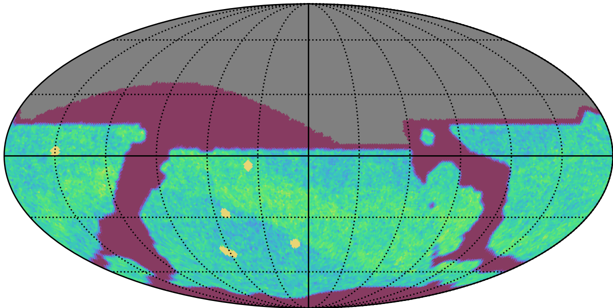
ddf_acor_sf10_lsf30_lsr50_v3.4_10yrs All sky i band: NVisits
