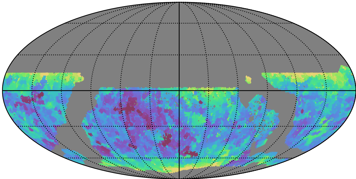
ddf_acor_sf10_lsf30_lsr50_v3.4_10yrs WFD y band: Min seeingEff
