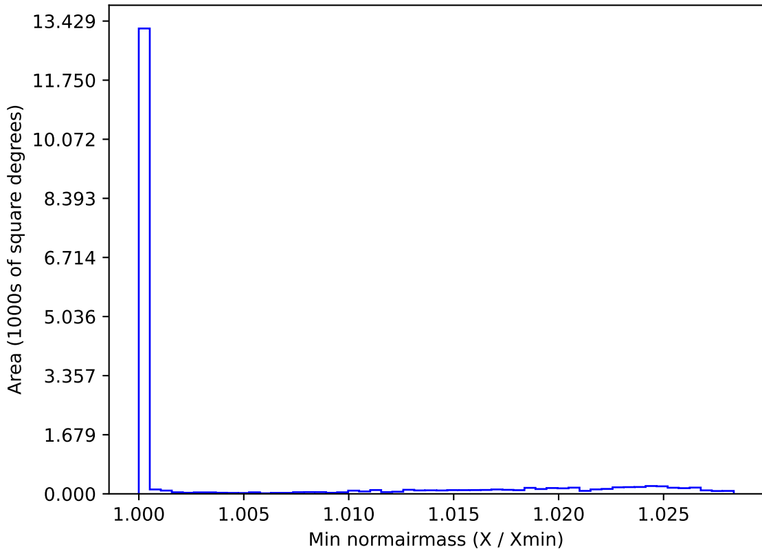
ddf_acor_sf10_lsf30_lsr50_v3.4_10yrs WFD all bands: Min normairmass
