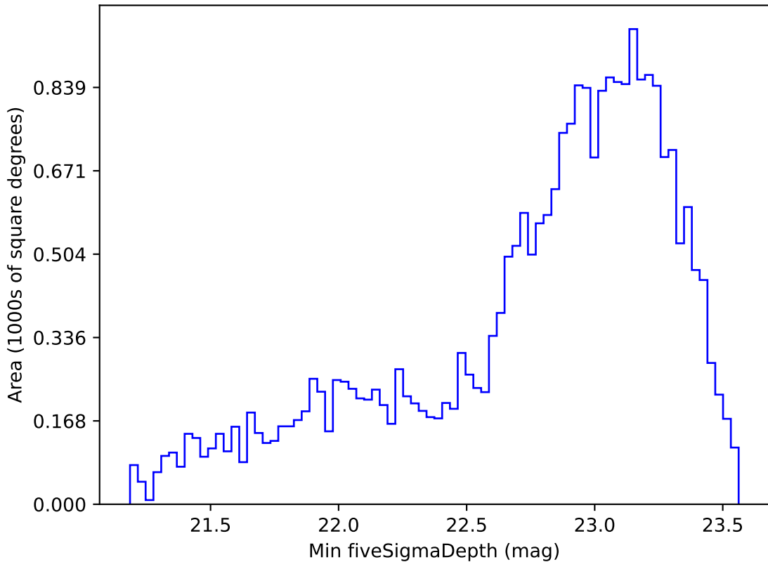
ddf_acor_sf10_lsf30_lsr50_v3.4_10yrs Yr 1 i band: Min fiveSigmaDepth
