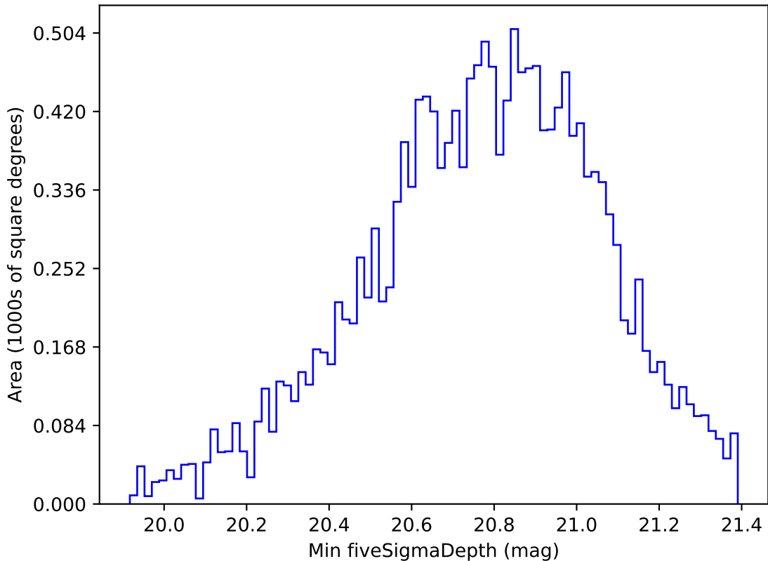
ddf_acor_sf10_ls30_lsr50_v3.4_10yrs WFD all bands: Min fiveSigmaDepth
