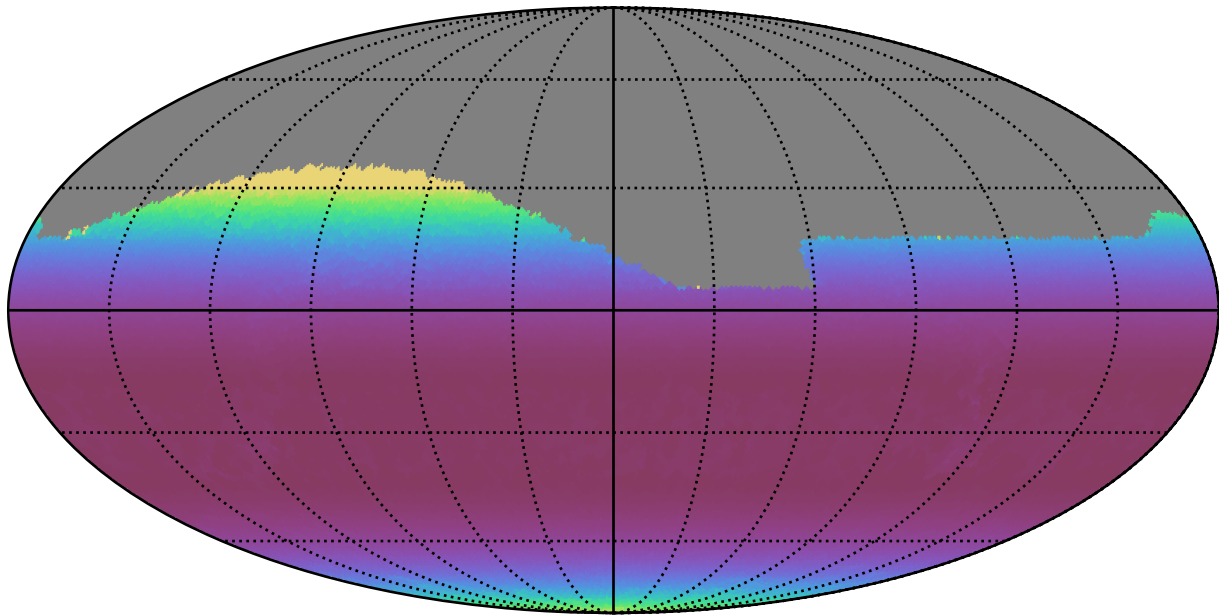
ddf_acor_sf10_lsf30_lsr50_v3.4_10yrs Yr 1 all bands: Min airmass
