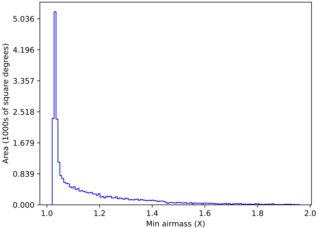
ddf_acor_sf10_lsf30_lsr50_v3.4_10yrs Yr 1 all bands: Min airmass
