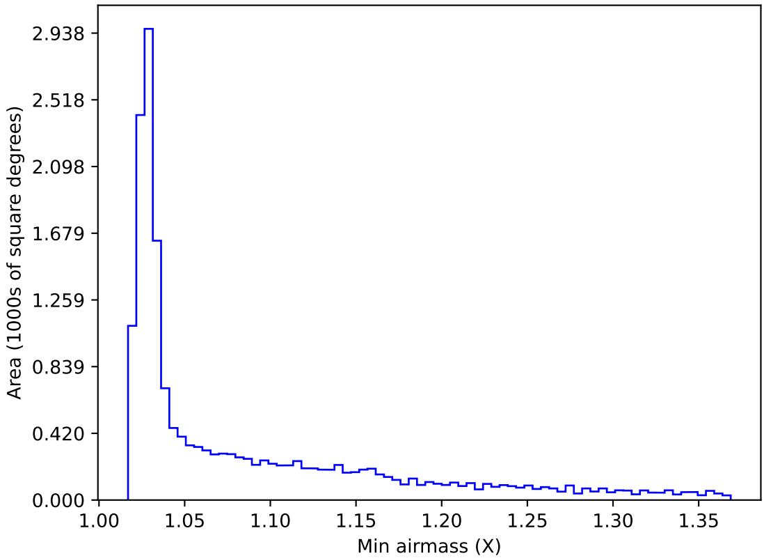
ddf_acor_sf10_lsf30_lsr50_v3.4_10yrs WFD r band: Min airmass
