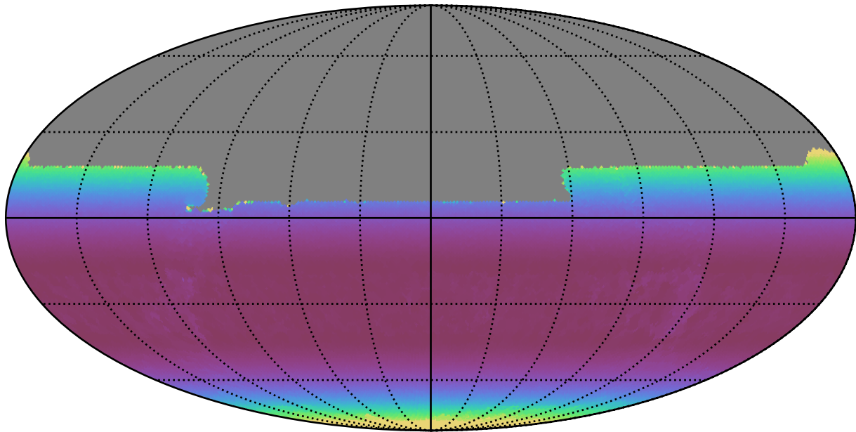
ddf_acor_sf10_lsf30_lsr50_v3.4_10yrs All sky y band: Min airmass
