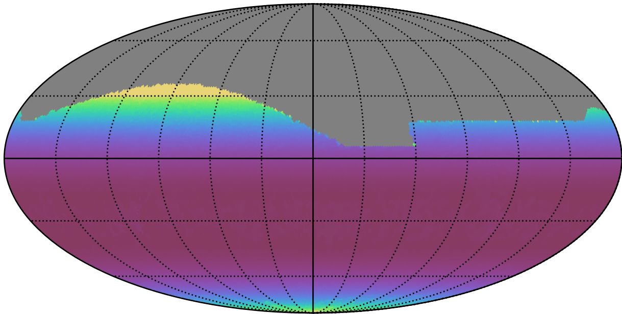
ddf_acor_sf10_lsf30_lsr50_v3.4_10yrs All sky r band: Min airmass
