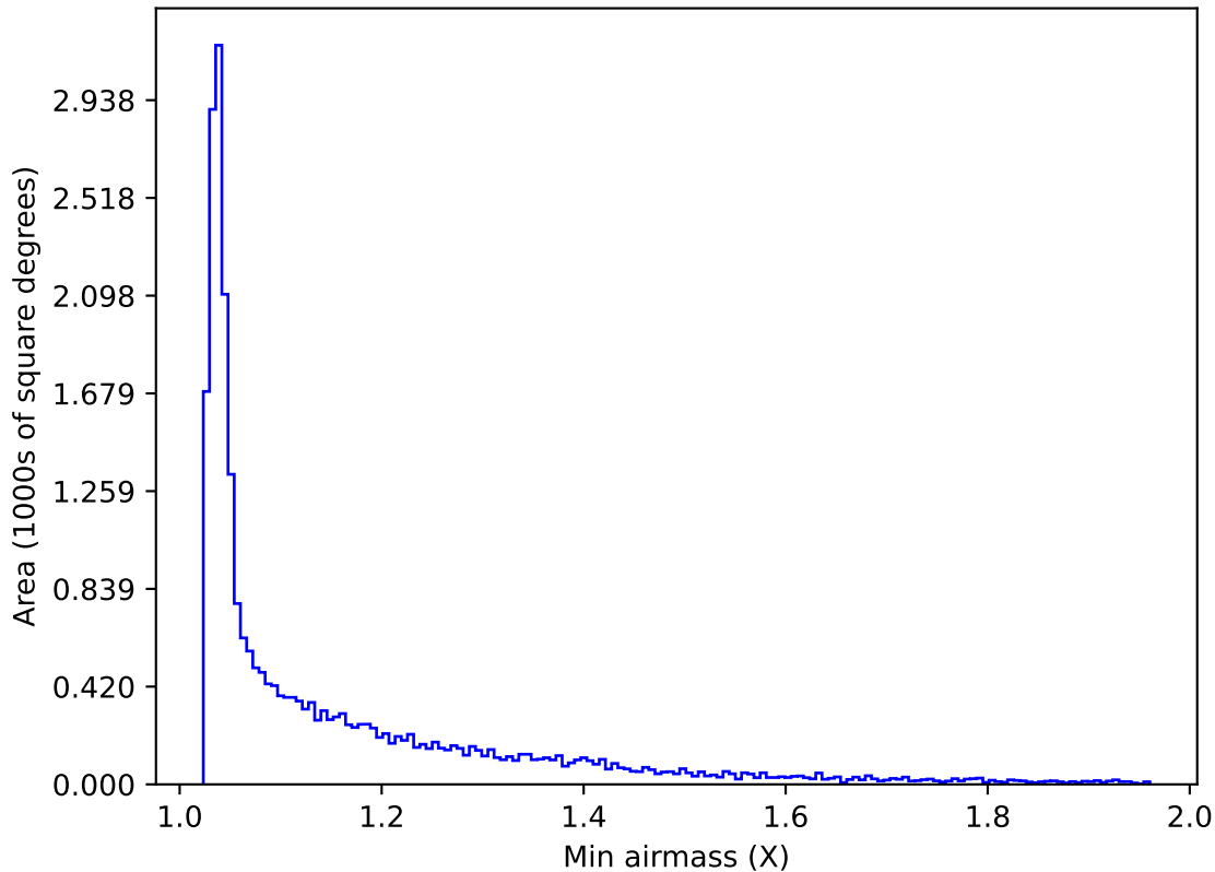
ddf_acor_sf10_lsf30_lsr50_v3.4_10yrs All sky g band: Min airmass
