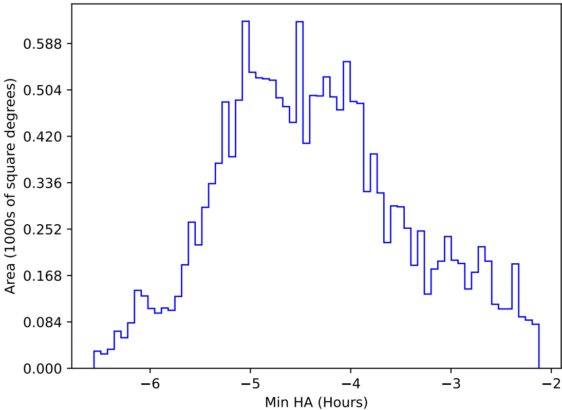
ddf_acor_sf10_lsf30_lsr50_v3.4_10yrs WFD i band: Min HA
