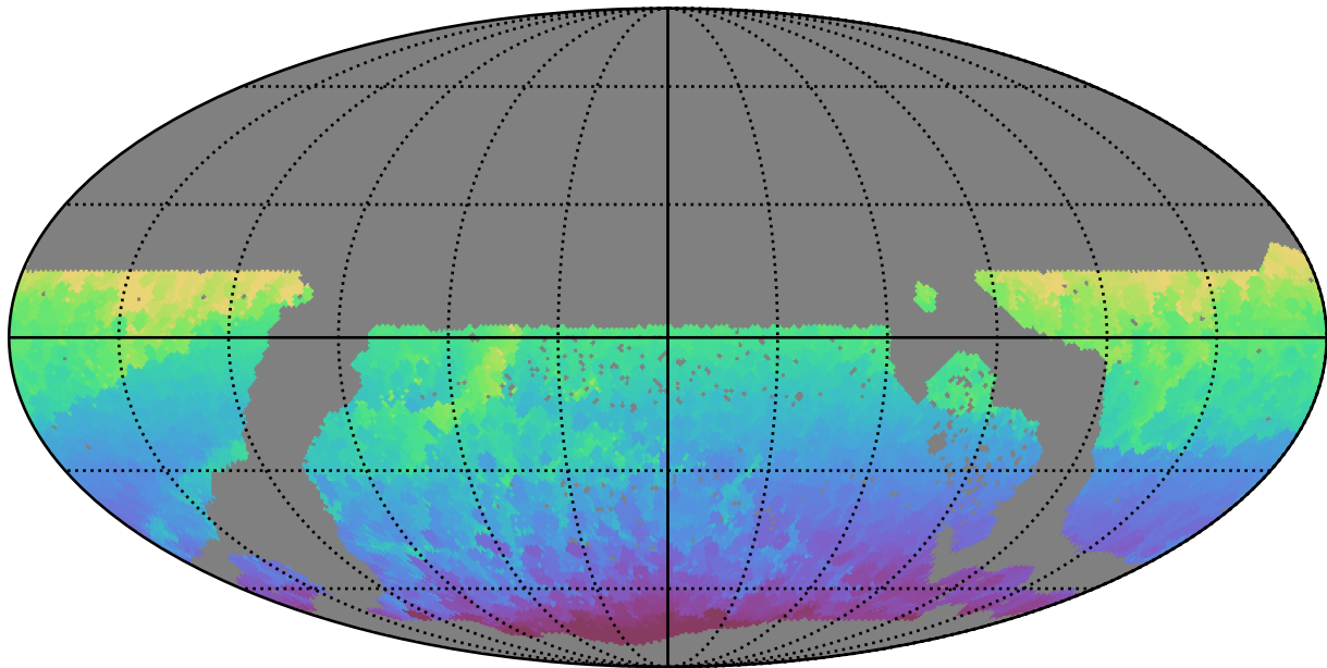
ddf_acor_sf10_lsf30_lsr50_v3.4_10yrs WFD all bands: Min HA
