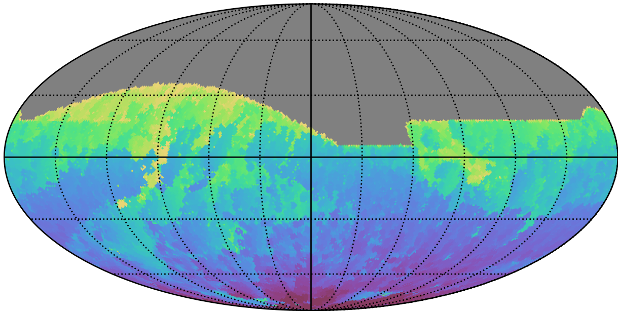
ddf_acor_sf10_lsf30_lsr50_v3.4_10yrs All sky z band: Min HA
