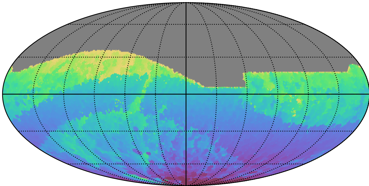
ddf_acor_sf10_lsf30_lsr50_v3.4_10yrs All sky r band: Min HA
