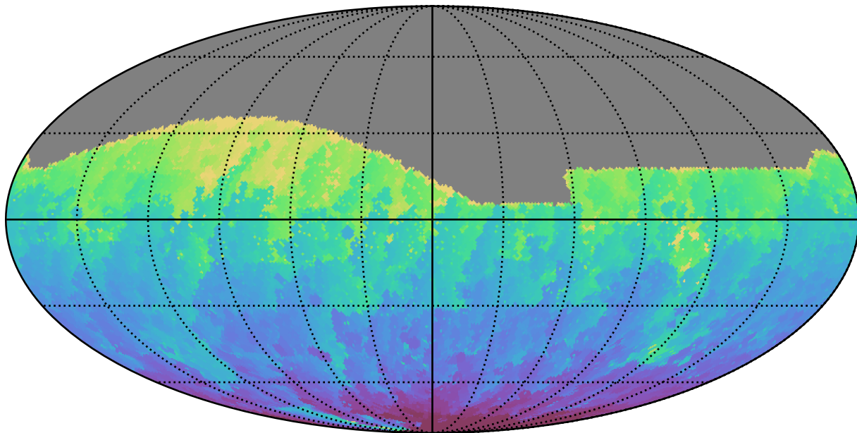
ddf_acor_sf10_lsf30_lsr50_v3.4_10yrs All sky g band: Min HA
