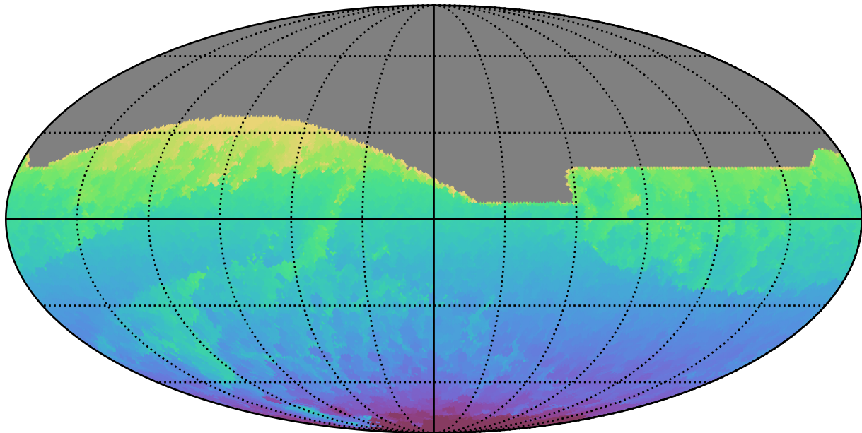
ddf_acor_sf10_lsf30_lsr50_v3.4_10yrs All sky all bands: Min HA
