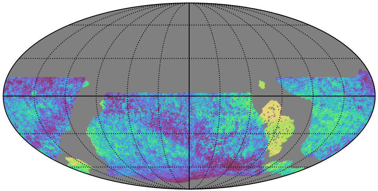
ddf_acor_sf10_lsf30_lsr50_v3.4_10yrs WFD all bands: Median skyBrightness
