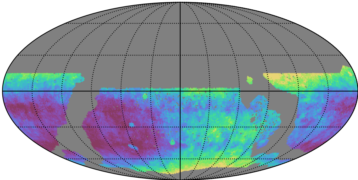
ddf_acor_sf10_lsf30_lsr50_v3.4_10yrs WFD i band: Median seeingEff
