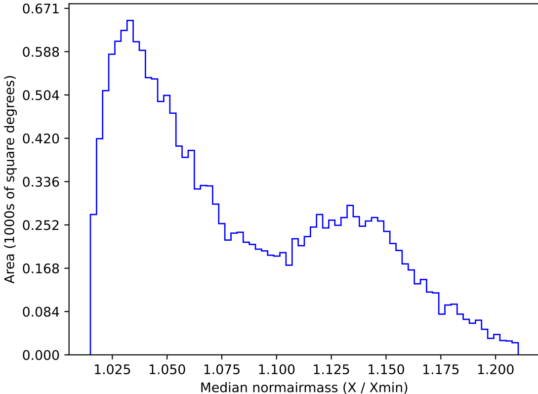
ddf_acor_sf10_lsf30_lsr50_v3.4_10yrs WFD g band: Median normairmass
